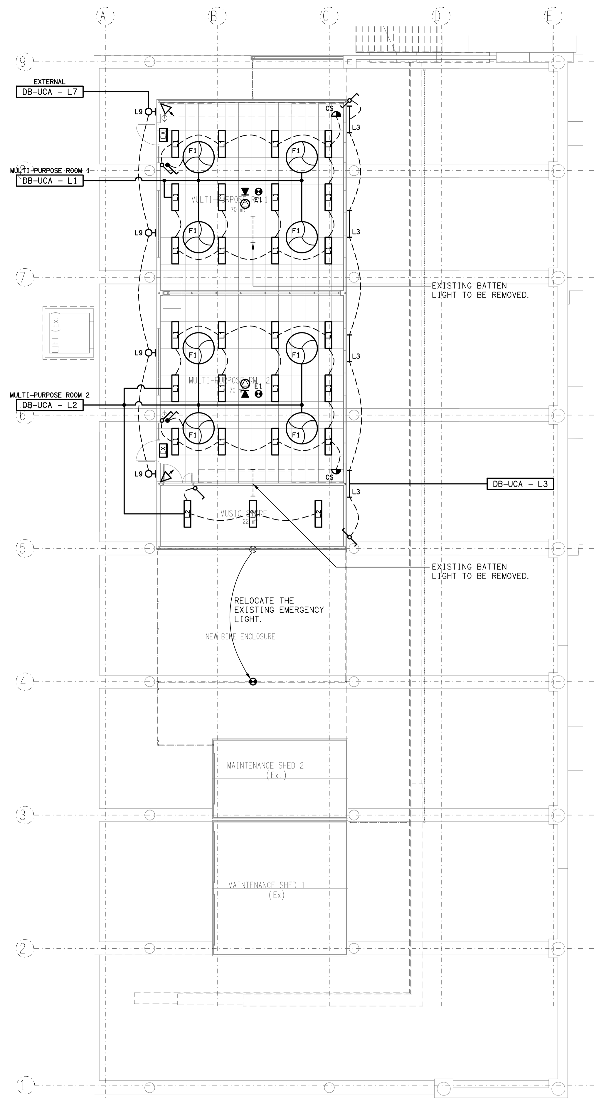
REFLECTED CEILING PLAN UNDERCROFT REFURBISHMENT SCALE 1:100
